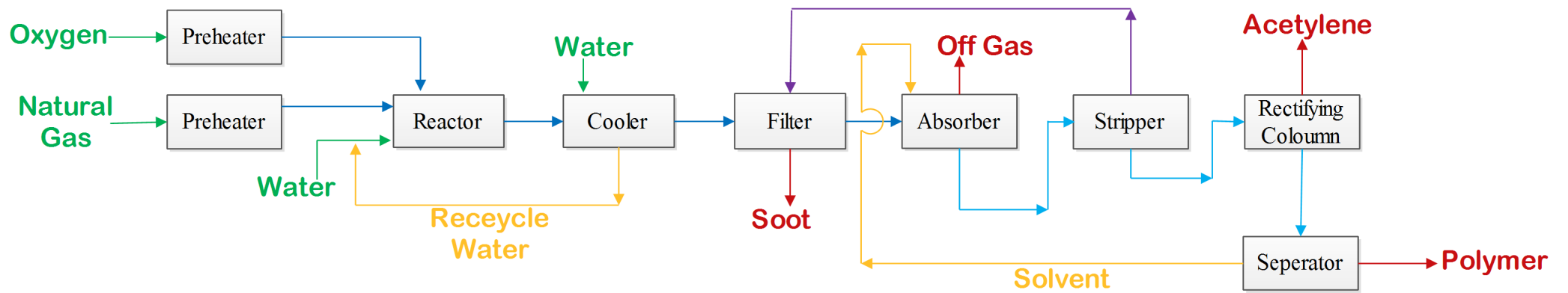
Figure: Manufacturing of Acetylene from Natural Gas
